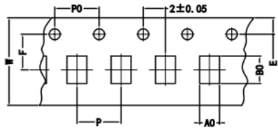
Tape Dimensions
