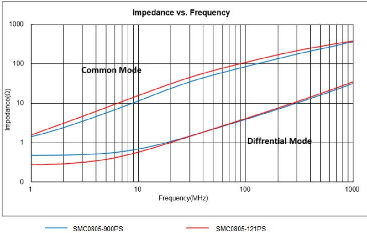
SMC0805 (90~120Ω)
